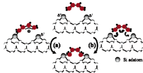
Scheme 1. Stepwise (a) and Concerted (b) Reaction Pathways of the [4+2]-Like Cycloaddition Reaction of 1,3-Butadiene on the Symmetric Si Adatom Pair
